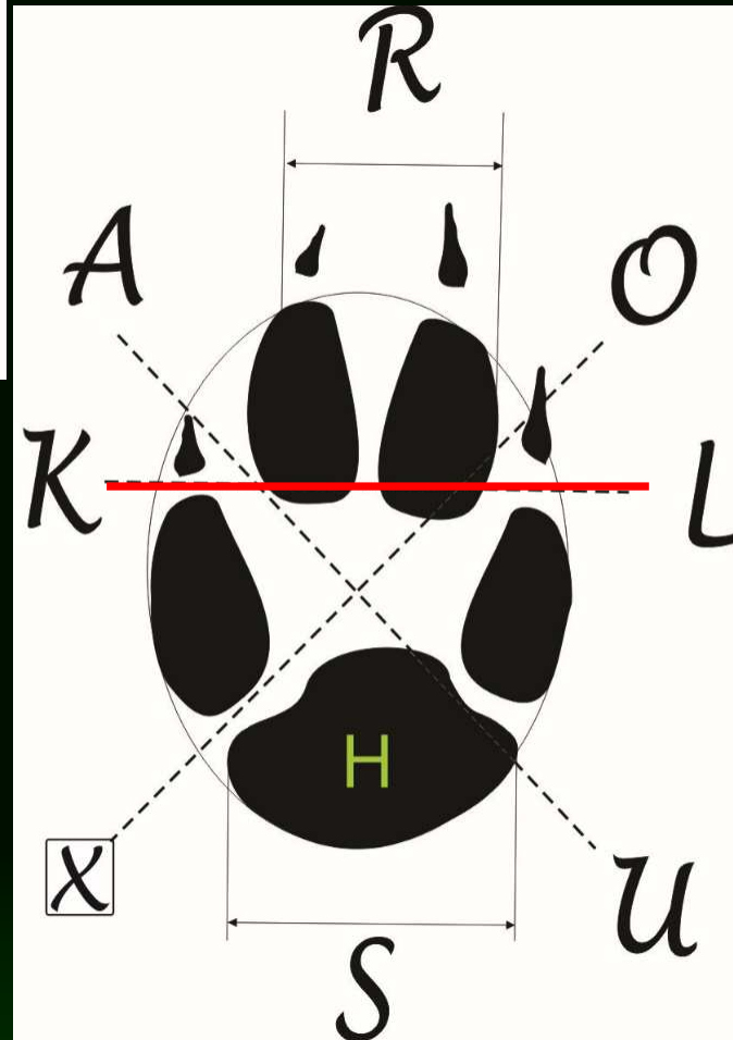
Hybrid
